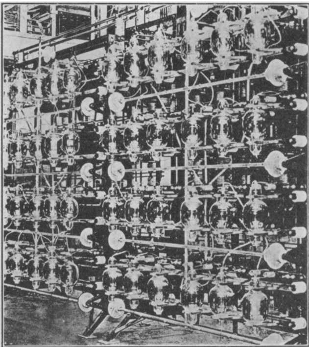
FIG. 1.—TUBE PANEL AT CARNARVON
