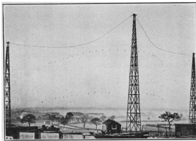
FIG. 5—DIRECTIONAL TRANSMITTER (HENDON)
