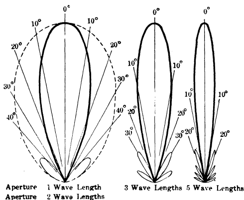
FIG. 4—CALCULATED POLAR CURVES OF REFLECTORS
