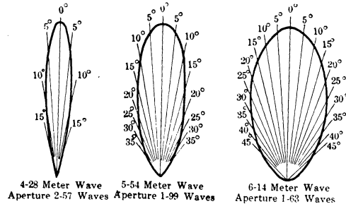
FIG. 10—POLAR CURVES OF INCHKEITH REFLECTOR
