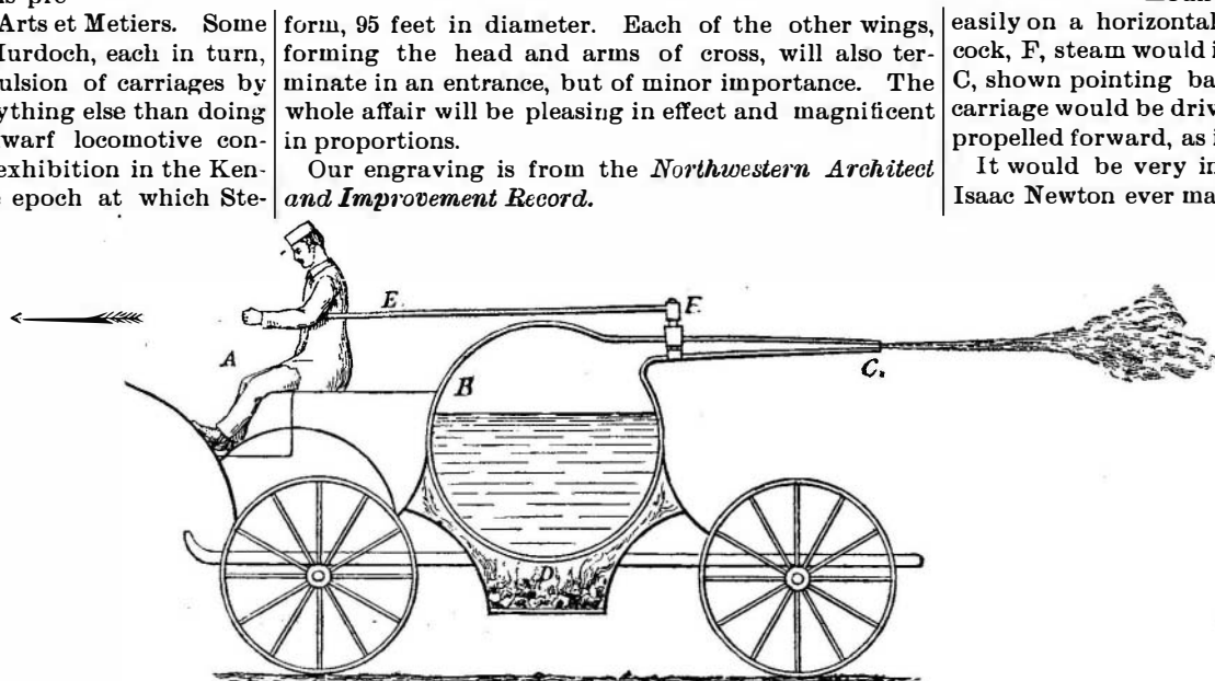
SIR ISAAC NEWTON'S STEAM CARRIAGE OF 1680.
